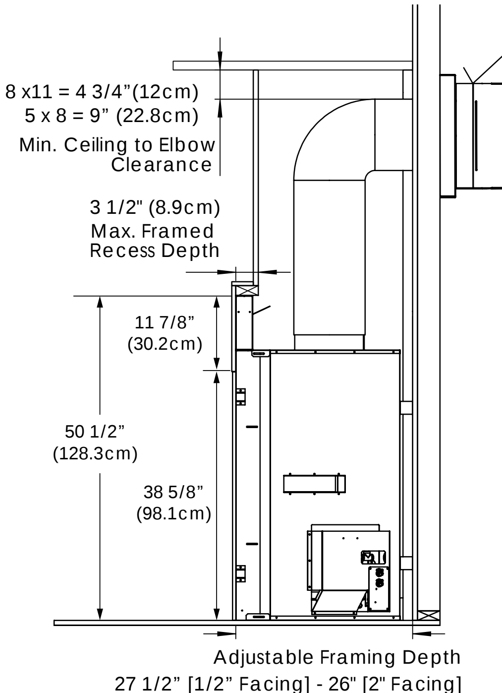
Figure 48: Recess Installation
