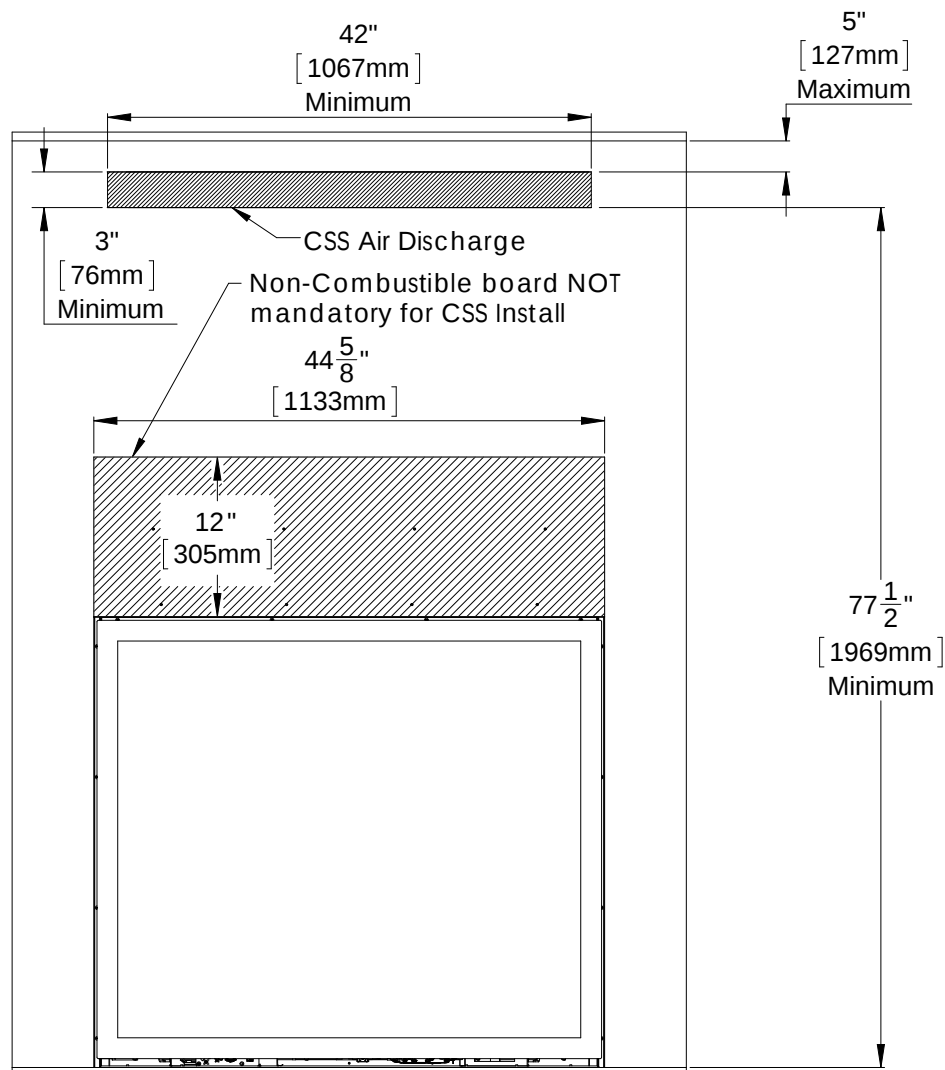
Figure 54: Typical Facing Layout
