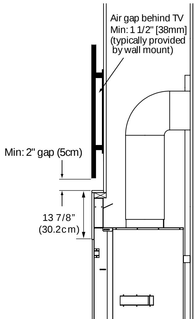
Figure 56: Recess Minimum TV Install
