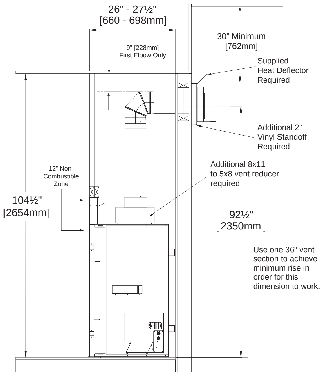
Figure 53: Minimum Vent - 5x8
