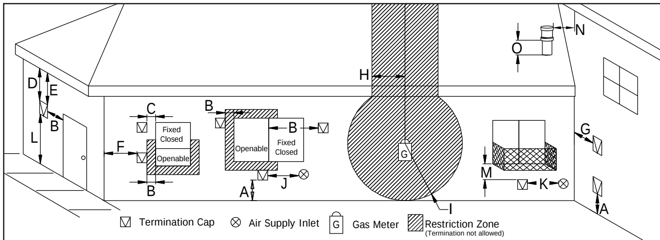
Figure 57: Vent Termination Restrictions, refer to Table 2
