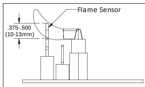
Figure 3: Pilot Light
