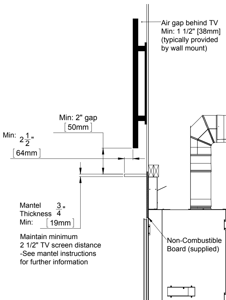
Figure 55: Minimum TV Install
