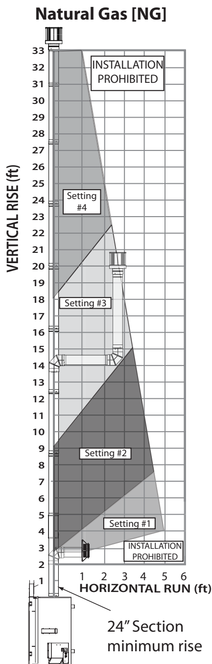
Figure 62: 8" x 11" NG Vent Graph
