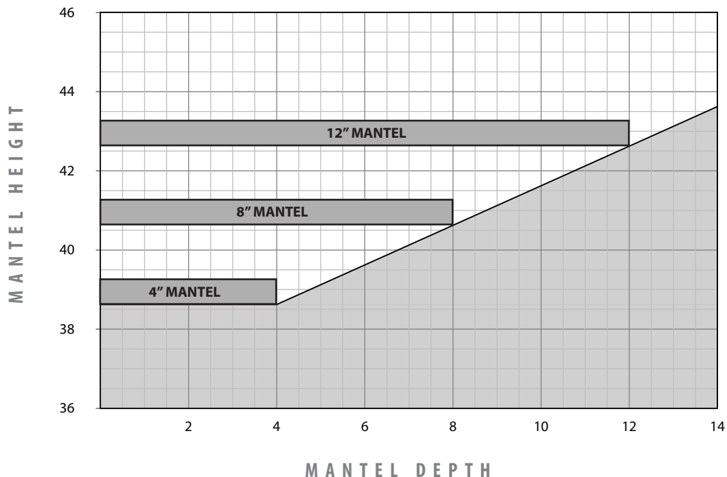
Figure 51: Mantel Clearances - CSS Activated
