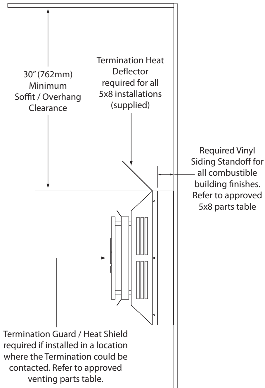
Figure 59: Additional Termination Restrictions for 5" x 8" Venting
