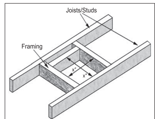
Figure 58: Thimble Framing
